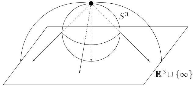
Figure 4.1: The stereographic projection identifies the three-sphere with the three-space compactified at spacial infinity, which is the image of the north pole.
