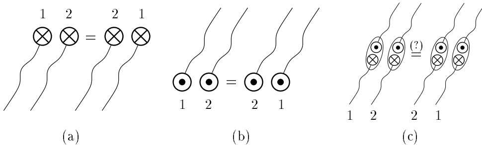
Figure 3.4: The two-particle-wave function of monopoles (a) and electric charges (b) is symmetric due to the fact that the charges do not feel string of their own kind. What will happen for bound states (c) is discussed in the text.
