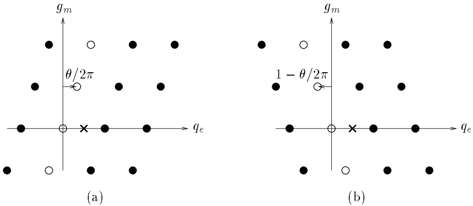
Figure 5.2: In the confinement phase all objects along a particular line in the charge lattice are free (○). Now electric objects like gluons (●) and quarks (x) are confined by vortices. The diagrams show the confinement phase for small \theta (a) and \theta near 2\pi (b). The switch inbetween refers to a phase transition.
