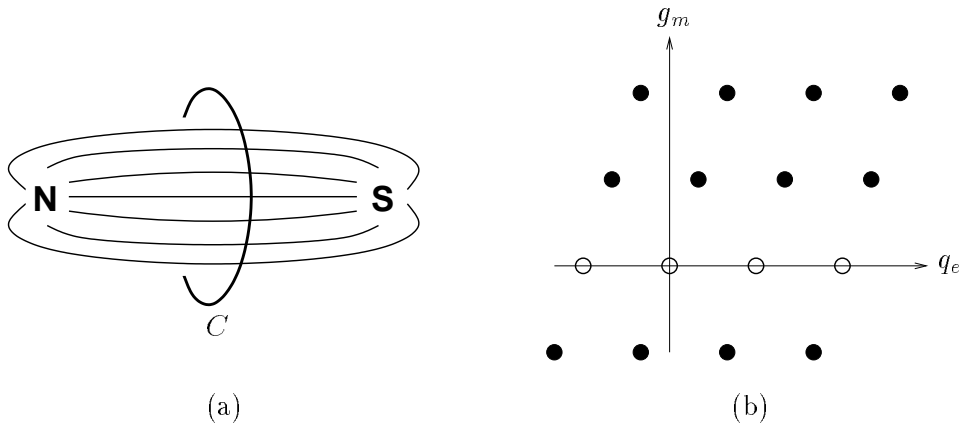
Figure 5.1: In the Higgs phase magnetic charges are connected by Meissner flux tubes. On the circle C the Higgs field makes a full rotation (a). In this phase all magnetic charges (●) are confined, while electric charges (○) are free/screened (b). This and the following gq diagrams refer to the simplest case of SU(2)_{\text{color}} .
