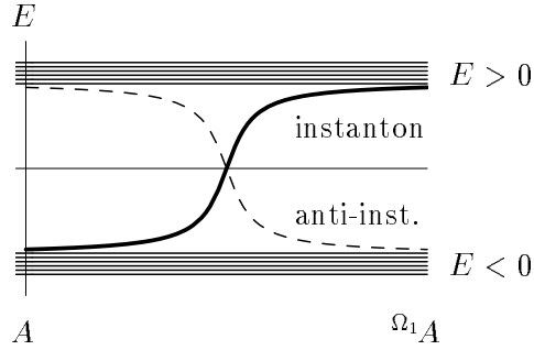
Figure 4.7: The instanton not only changes the winding number by 1, but also creates a (left-handed) particle and removes a (right-handed) anti-particle. For the anti-instanton it is vice versa. Infact the picture is delicate: In the original theory there is no mass and no gap, but we could add a small mass and the considerations still hold.
