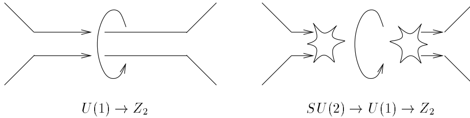
Figure 2.8: The snapping of vortices (see text).
